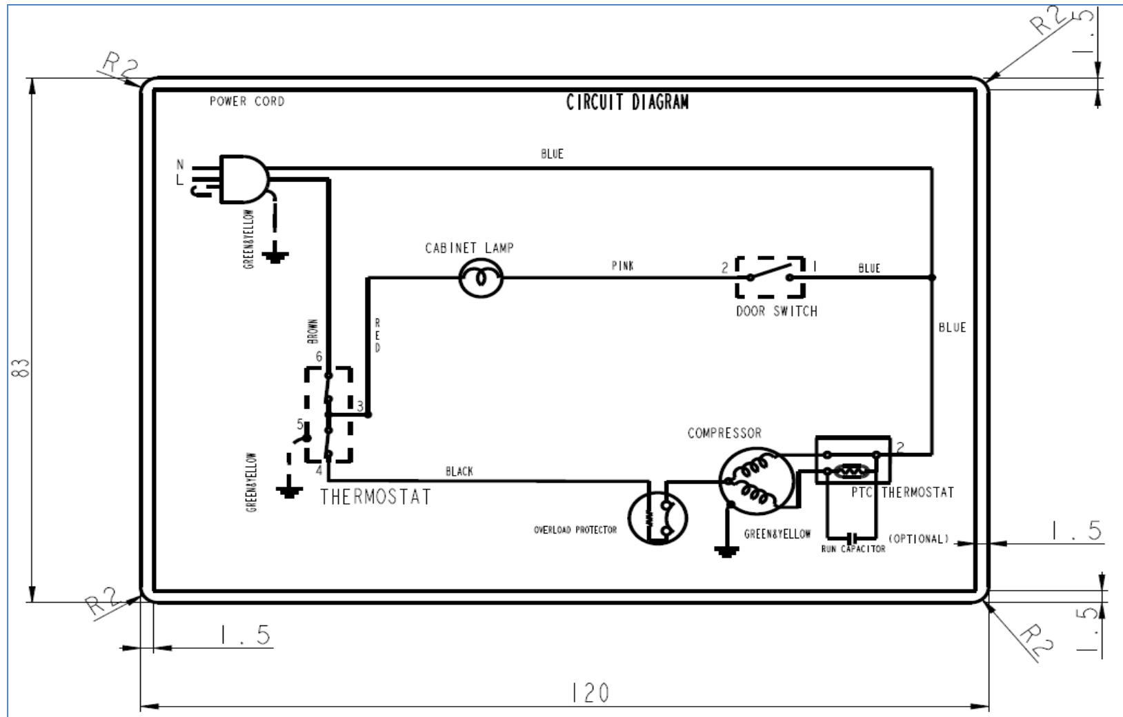
RBL6 Wiring Diagram
