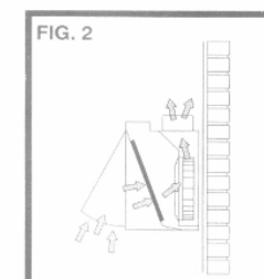
FIG. 2 RECIRCULATING MODE (CHARCOAL FILTERS REQUIRED)
