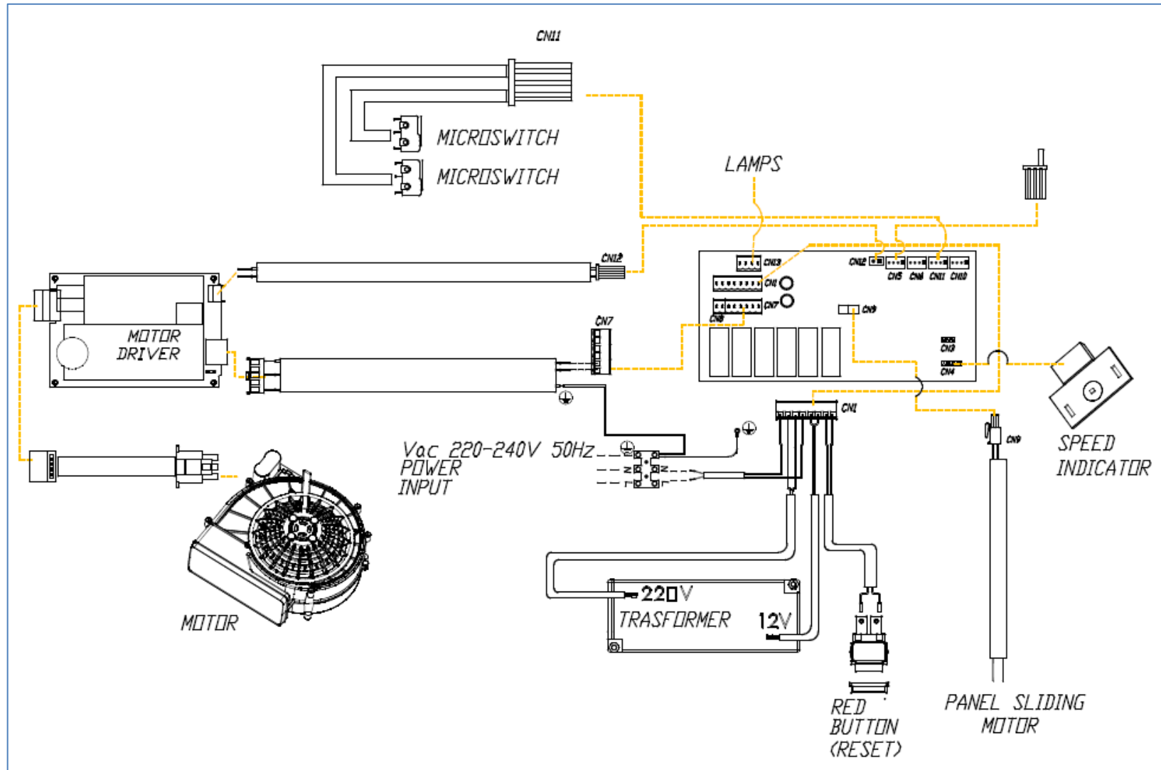
CE930 Wiring Diagram
