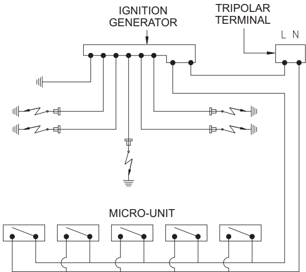
ELECTRIC DIAGRAM 5 BURNERS
