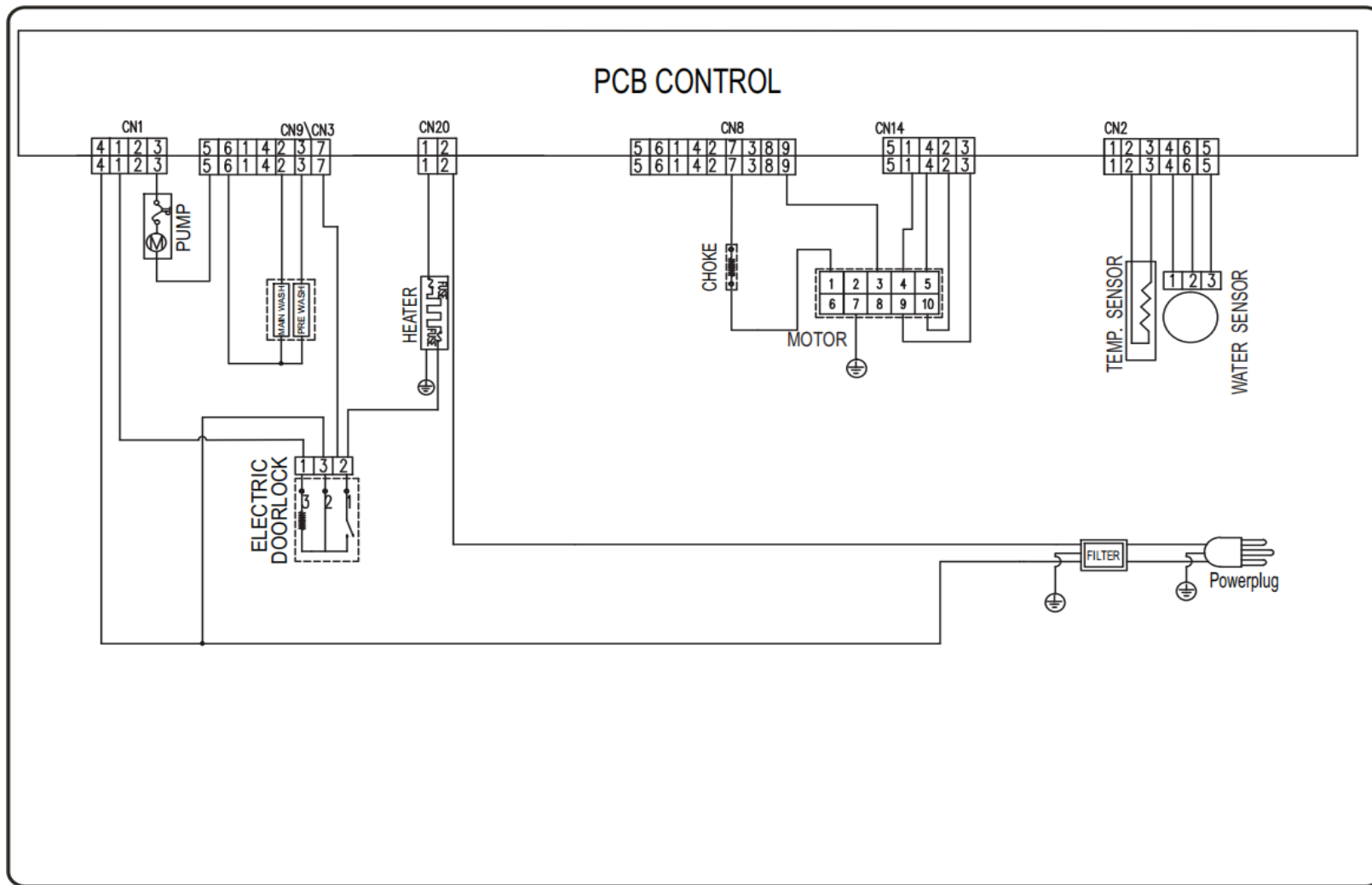
WMI3007 Wiring Diagram
